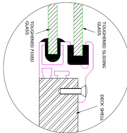
TYPICAL DETAILS FOR SLIDING GLASS WINDOW
