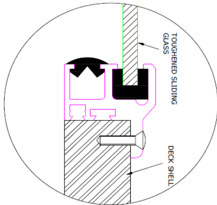
TYPICAL DETAILS FOR FIXED GLASS WINDOW
